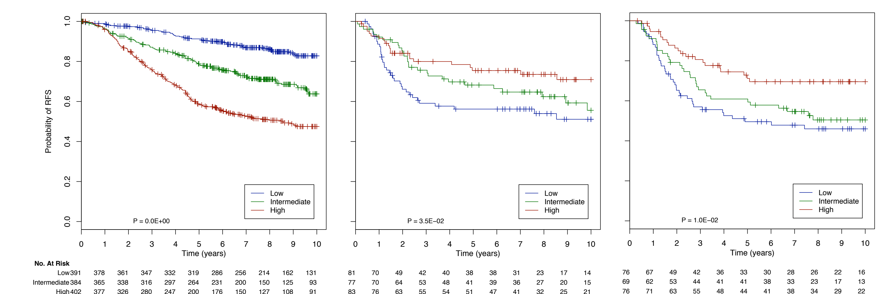
Figure 3: Kaplan-Meier curves for most relevant features in each BC subtype.
