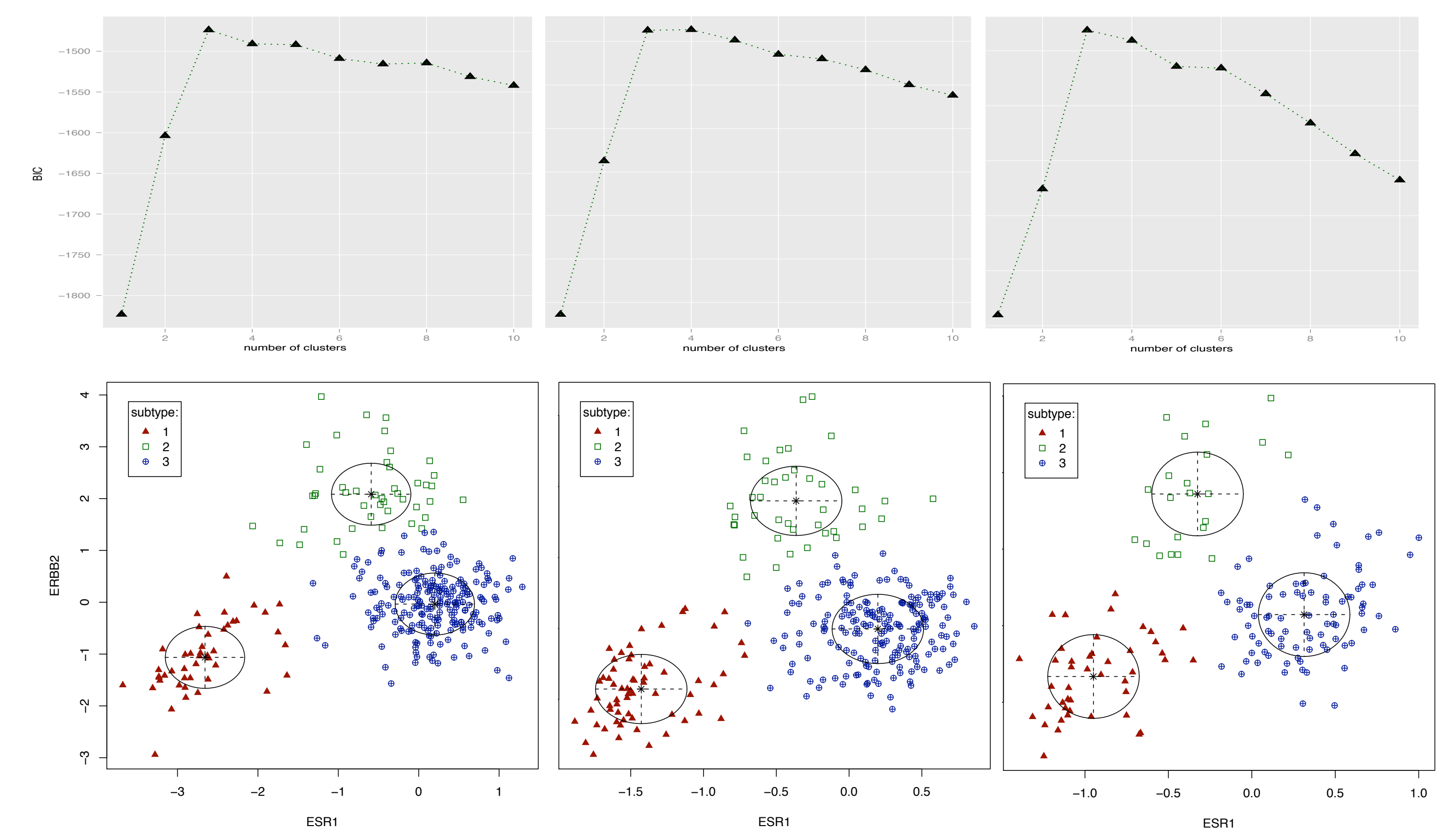
Figure 2: BC subtypes in NKI2, VDX and UNC datasets respectively.
