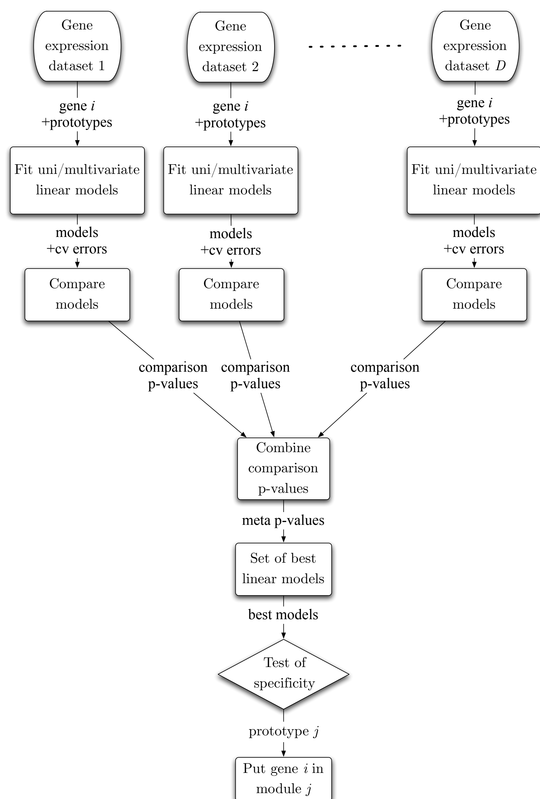
Figure 1: Prototype-based clustering method in a meta-analytical framework.
