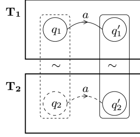
Fig. 2. Backward stable relation
